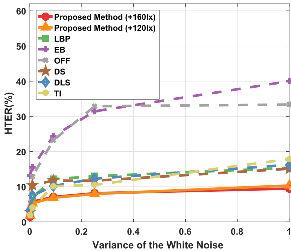
Fig. 9. Average HTER (%) of the proposed methods with +120lx and +160lx, and the comparison methods on images contaminated by the white noise with difference variances.
