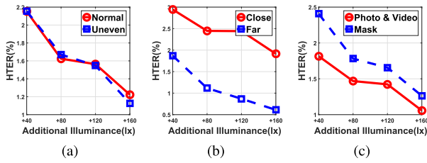
Fig. 8. The change of average HTER (%) of the proposed method under different settings and attack types: (a) Under normal and uneven illuminance; (b) Under close and far background distance; (c) Under photo & video and mask attacks.
