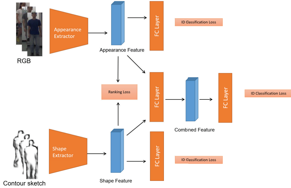
FIGURE 1. The architecture of our proposed dual-path model. The appearance and shape extractors measure RGB and contour sketch person images respectively. The concatenated appearance and shape features are fed into an FC layer to obtain the output.
