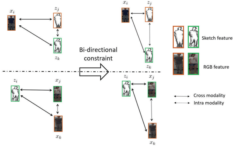
FIGURE 2. The illustration of the ranking loss. The ranking loss aims to push negative RGB-sketch pairs and pull positive RGB-sketch pairs. x and z denotes the RGB and sketch features, and the same border color denotes the same person identity.
