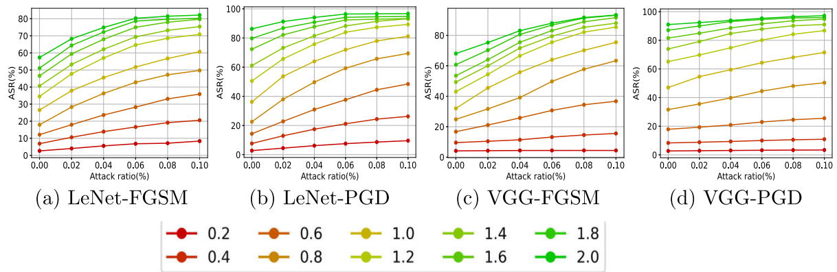
Fig. 4. ASR of the models (LeNet and VGG) under the indiscriminate adversarial attacks (FGSM and PGD) with different perturbation limitations represented by different colors on MNIST.
